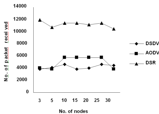
Figure 1: Packet Received for Protocols over Nodes
