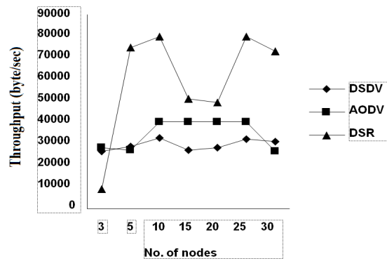
Figure 2: Throughput of Protocols over Nodes
