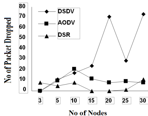
Figure 3: Packet Dropping for Protocols over Increasing Nodes
